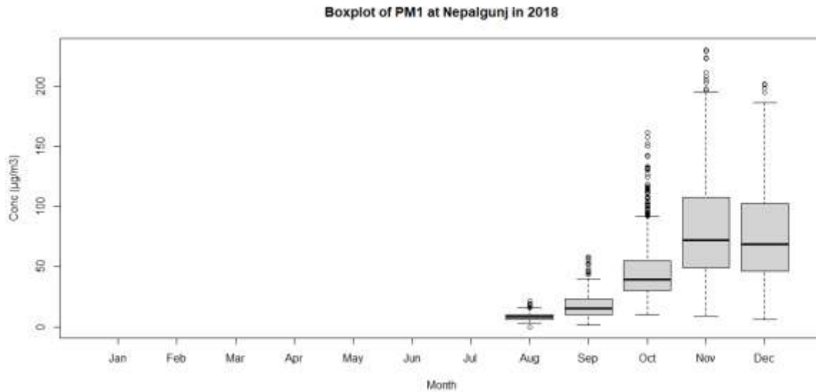
Figure 5: Monthly Variation of PM 1 in 2018
