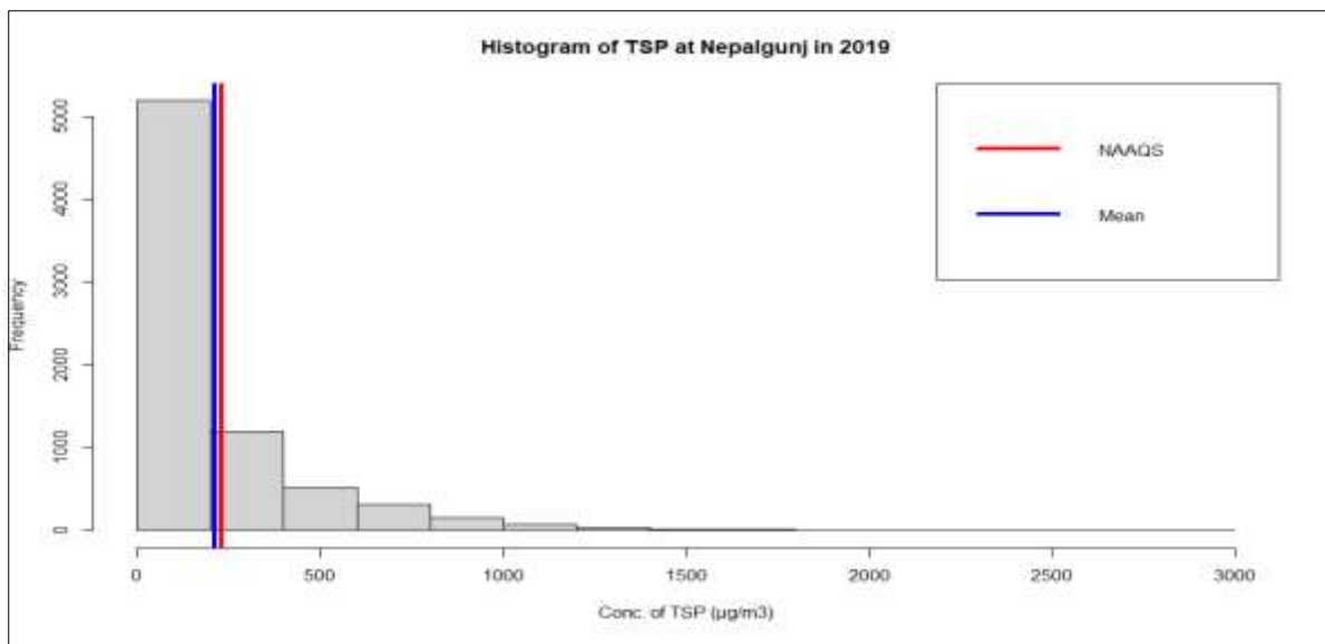
Figure 46: Histogram for the ambient concentration of TSP
