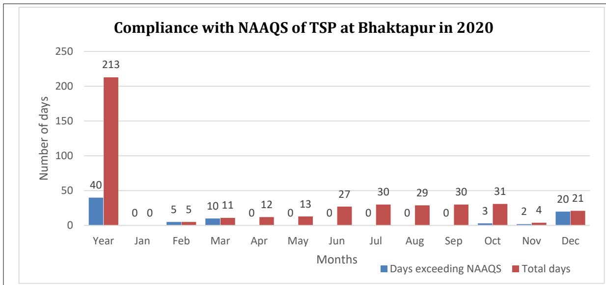
Figure 80: Compliance status of TSP
