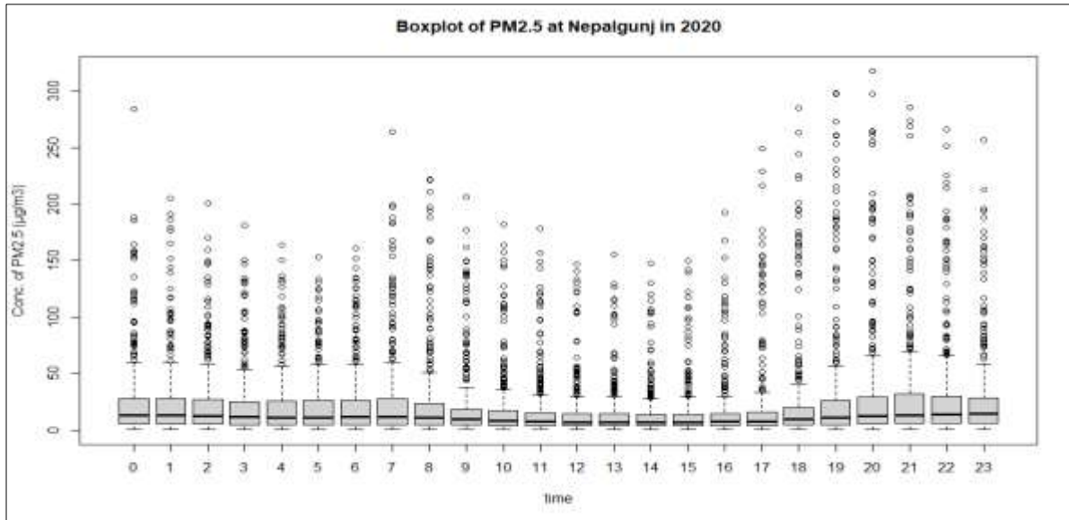
Figure 65: Diurnal variation of average PM 2.5 concentration
