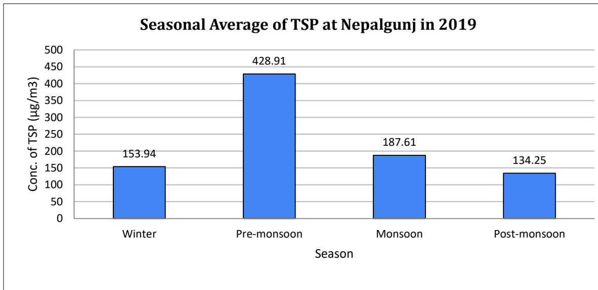
Figure 50: Seasonal variation of TSP
