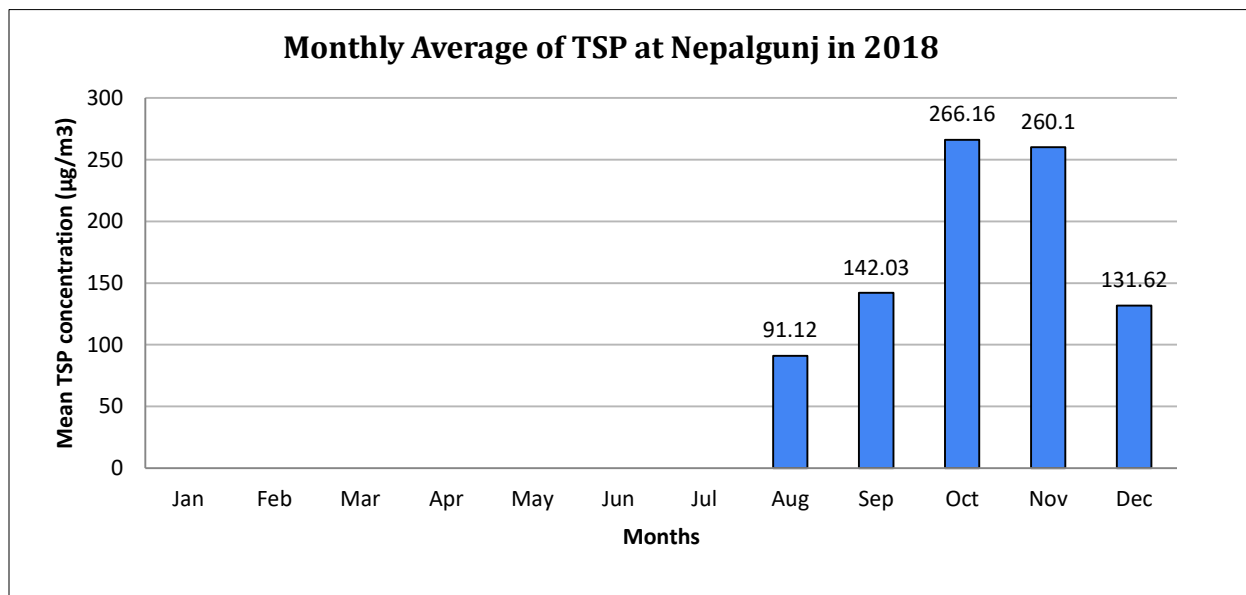
Figure 21: Monthly average of TSP
