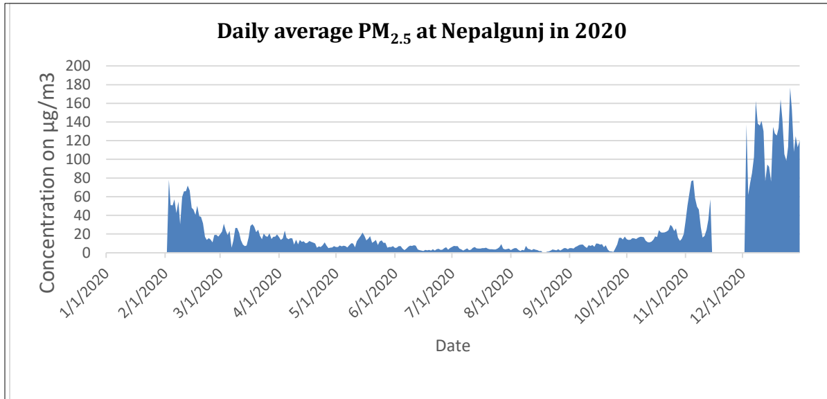
Figure 61: Daily average of PM 2.5 in 2020
