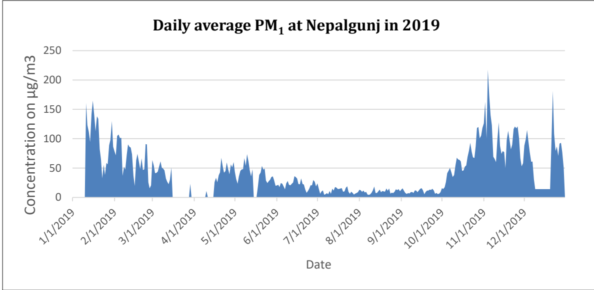
Figure 27: Daily average of PM 1
