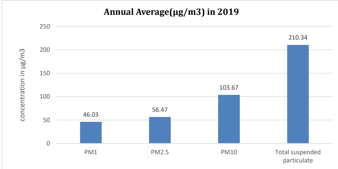
Figure 25: Annual average of PM 1 , PM 2.5 , PM 10 and TSP in 2019
