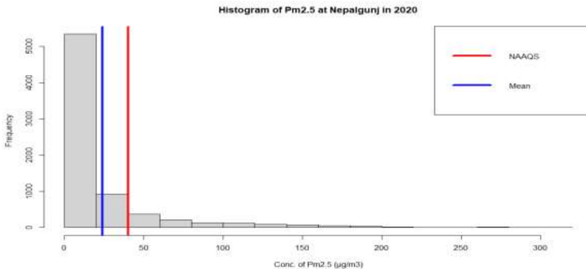
Figure 60 : Histogram for the ambient concentration of PM 2.5
