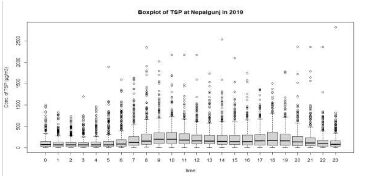
Figure 51: Diurnal variation of average TSP concentration
