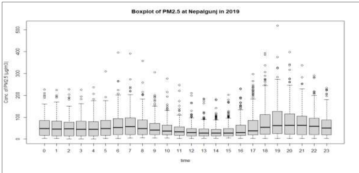
Figure 37: Diurnal variation of average PM 2.5 concentration
