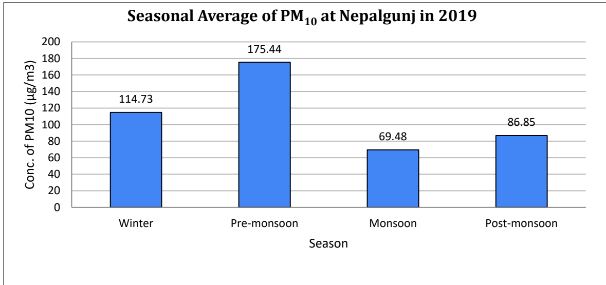
Figure 43: Seasonal variation of PM 10
