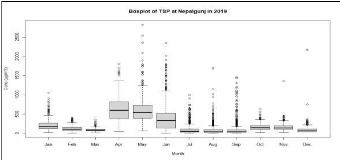
Figure 49: Monthly Variation of TSP
