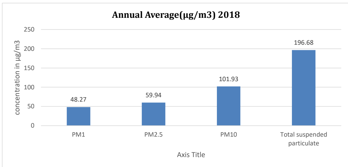
Figure 1: Annual average of PM 1 , PM 2.5 , PM 10 and TSP in 2018
