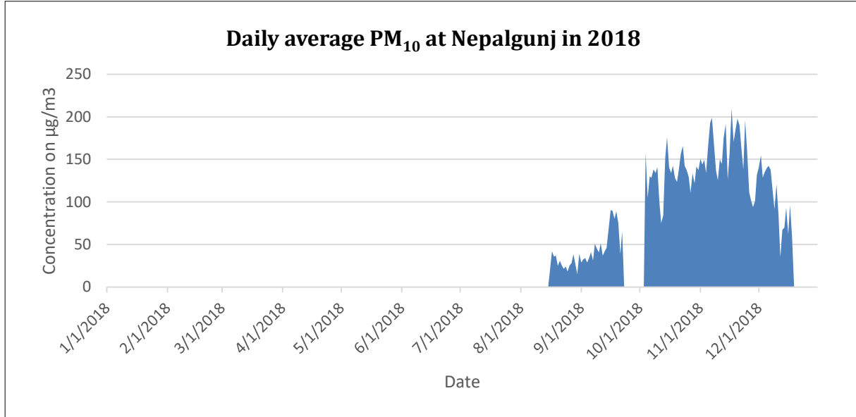
Figure 14: Daily average of PM 10
