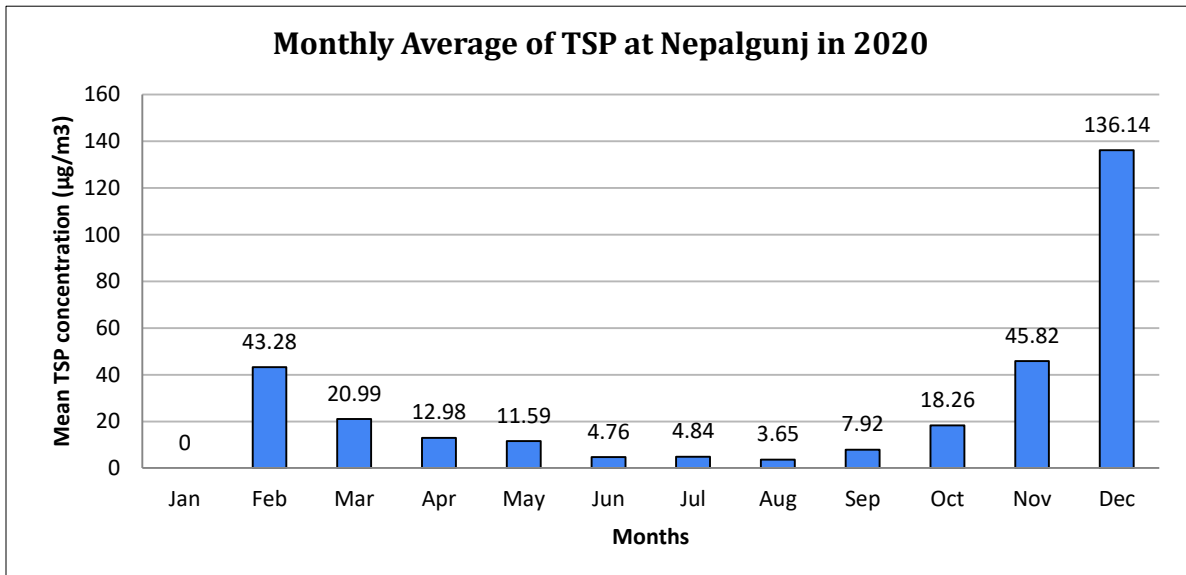
Figure 76: Monthly average of TSP
