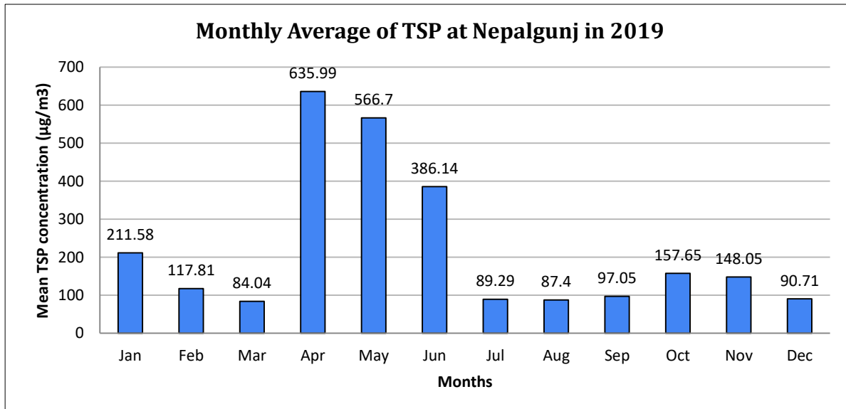
Figure 48: Monthly average of TSP
