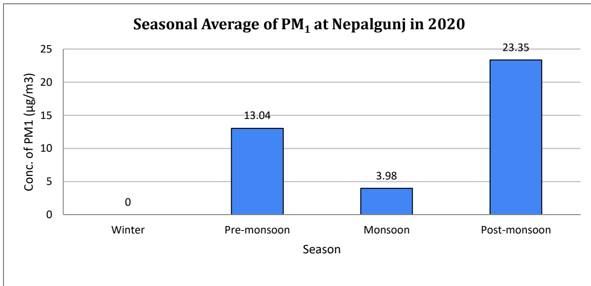
Figure 58: Seasonal variation of PM 1
