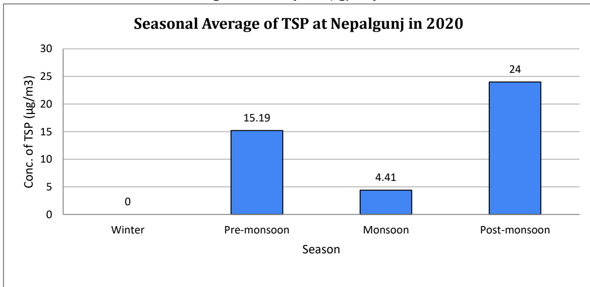
Figure 78: Seasonal variation of TSP
