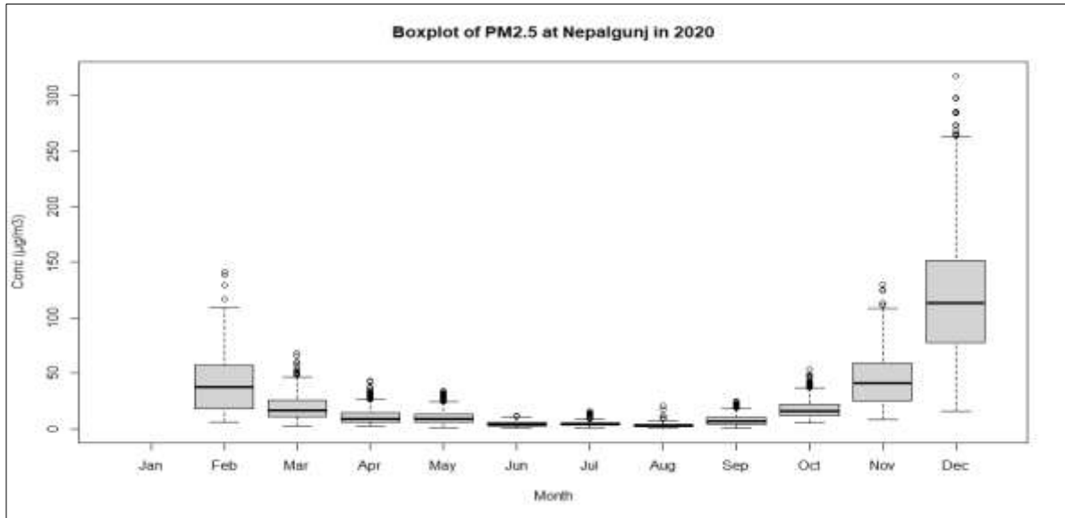
Figure 63: Monthly Variation of PM 2.5
