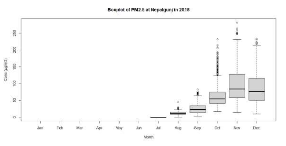
Figure 10: Monthly Variation of PM 2.5
