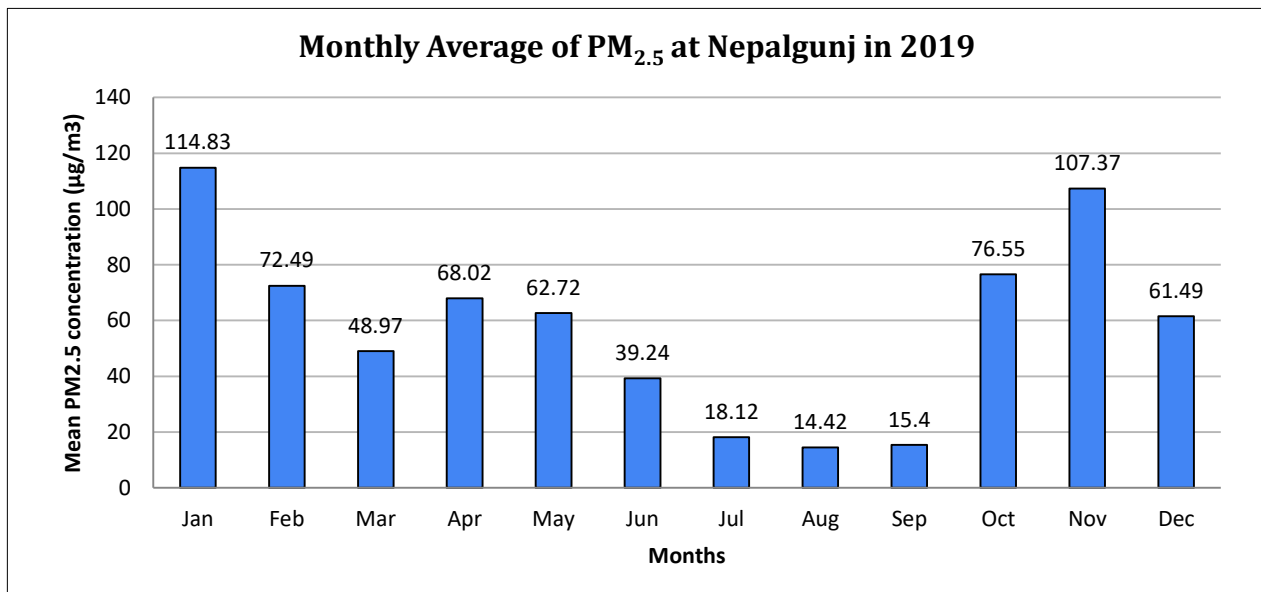
Figure 34: Monthly average of PM 2.5
