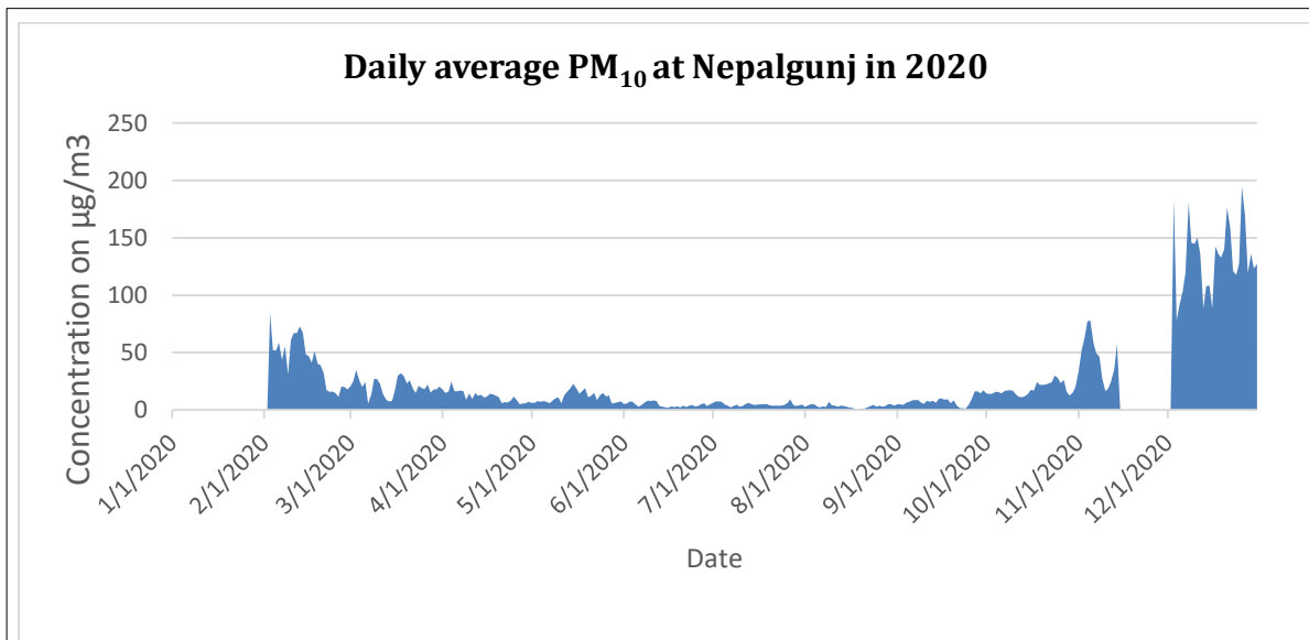
Figure 68: Daily average of PM 10
