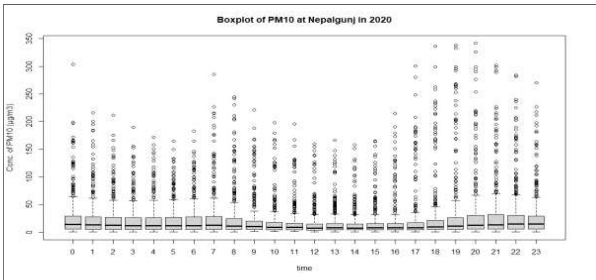
Figure 72: Diurnal variation of average PM 10 concentration
