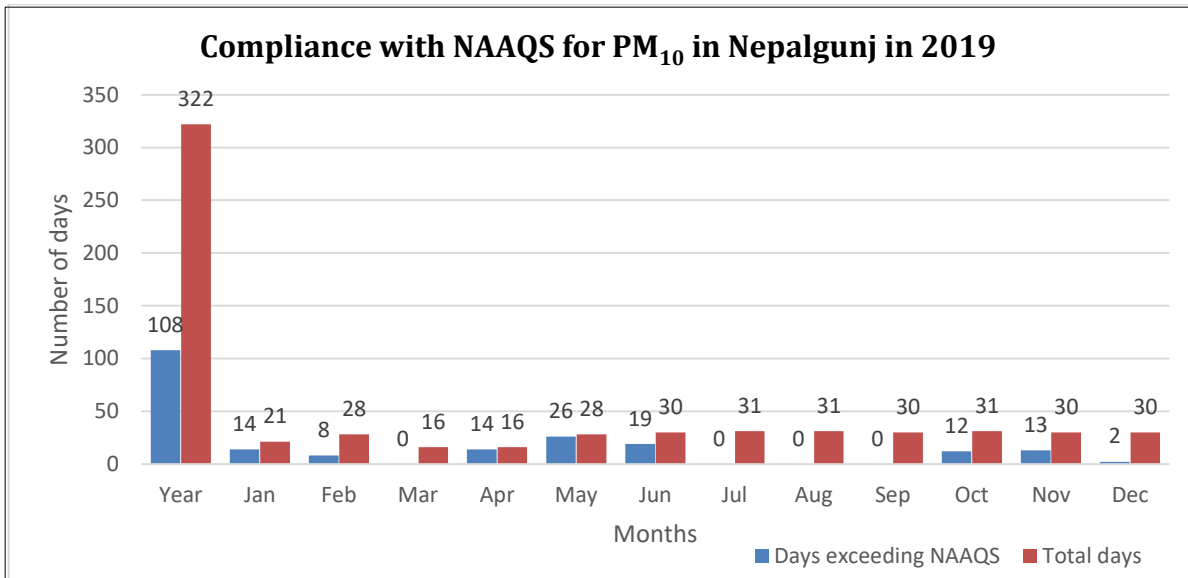
Figure 45: Compliance status of PM 10
