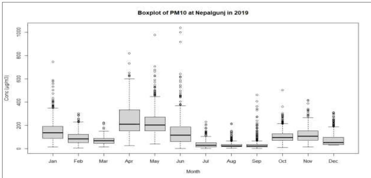
Figure 42: Monthly Variation of PM 10
