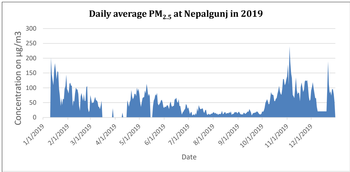
Figure 33: Daily average of PM 2.5 in 2019
