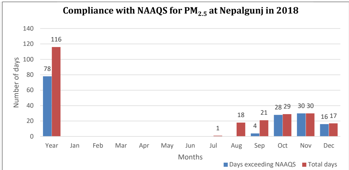
Figure 12: Compliance status of PM 2.5
