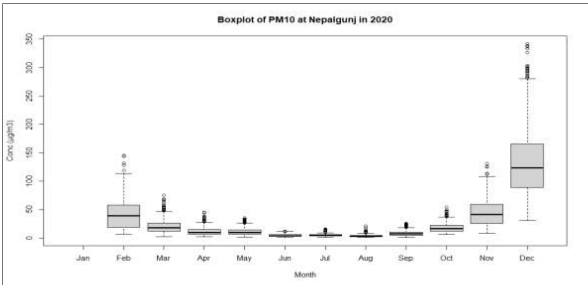
Figure 70: Monthly Variation of PM 10
