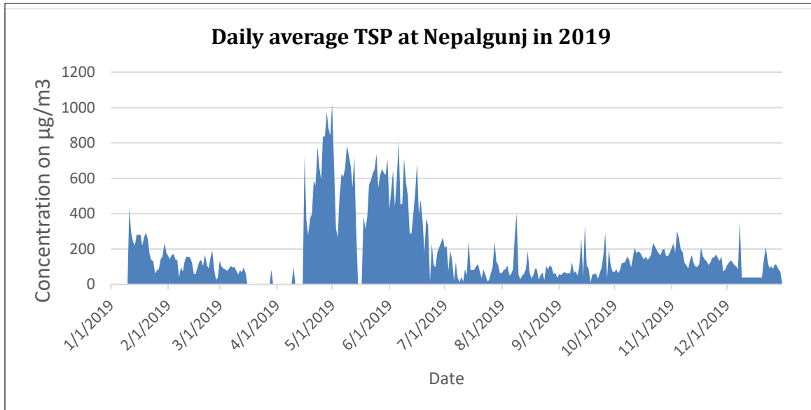
Figure 47: Daily average of TSP in 2019
