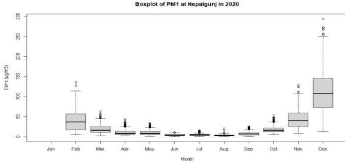
Figure 57: Monthly Variation of PM 1
