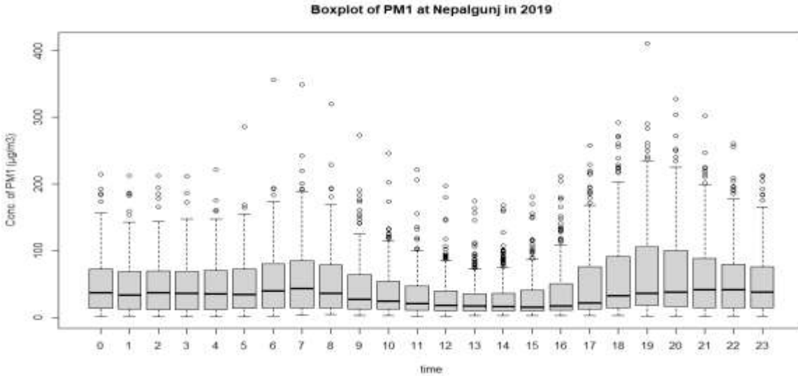
Figure 31: Diurnal variation of average PM 1 concentration
