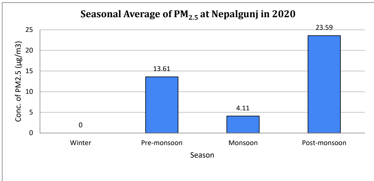
Figure 64: Seasonal variation of PM 2.5
