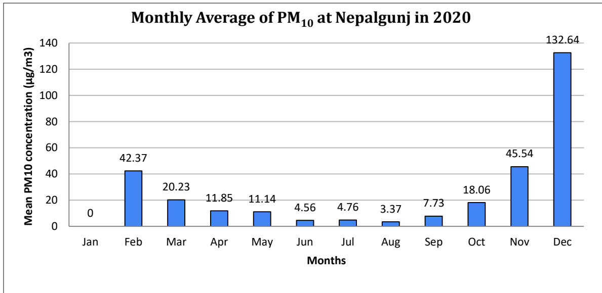
Figure 69: Monthly average of PM 10
