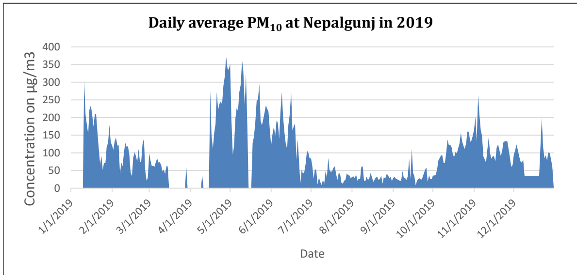
Figure 40: Daily average of PM 10
