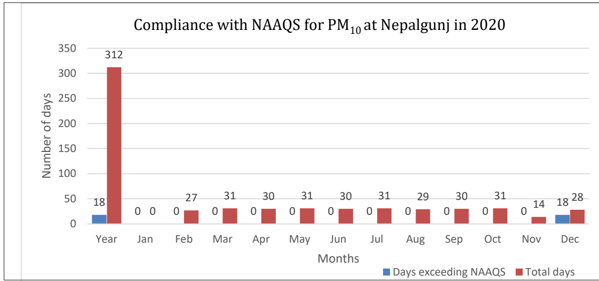
Figure 73: Compliance status of PM 10
