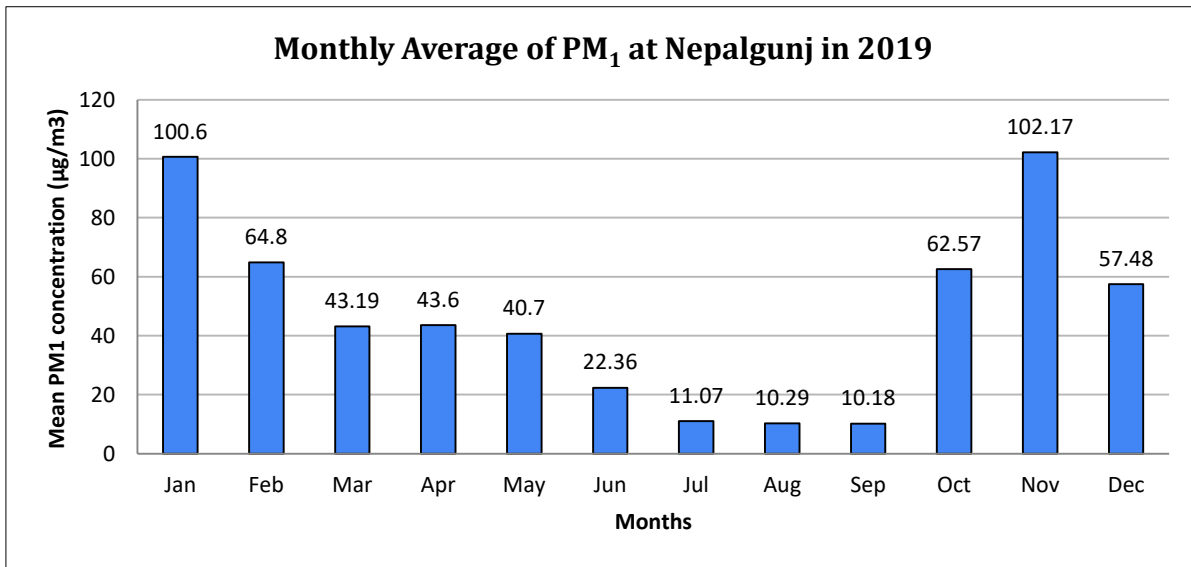
Figure 28: Monthly average of PM 1
