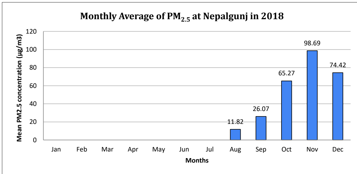
Figure 9: Monthly average of PM 2.5
