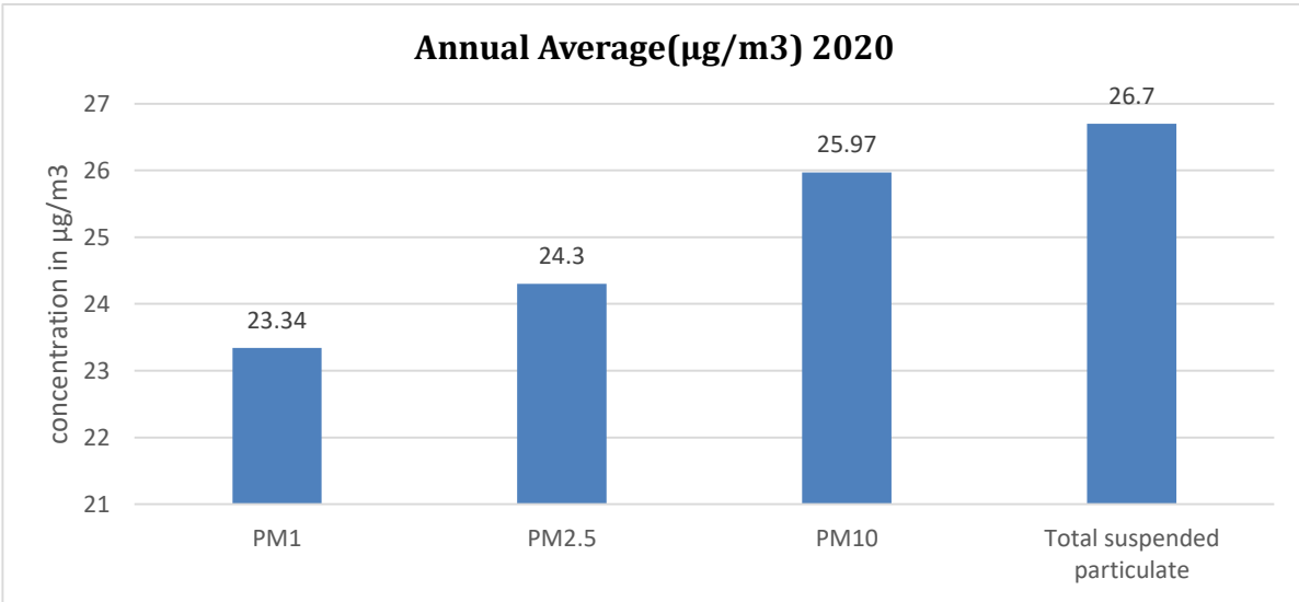
Figure 53: Annual average of PM 1 , PM 2.5 , PM 10 and TSP in 2020
