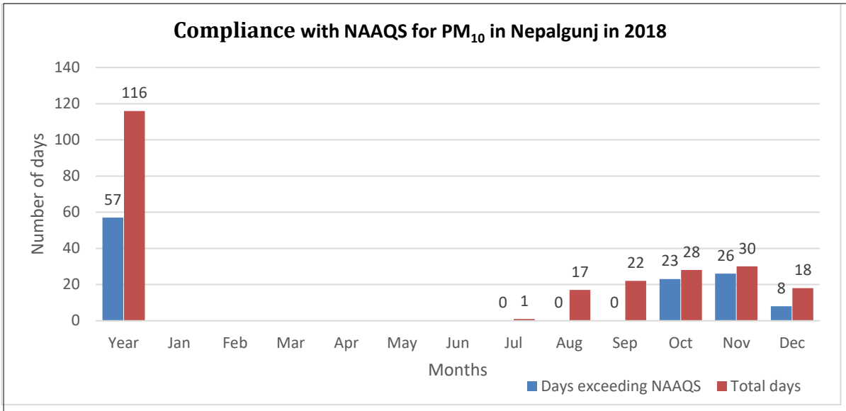
Figure 18: Compliance status of PM 10
