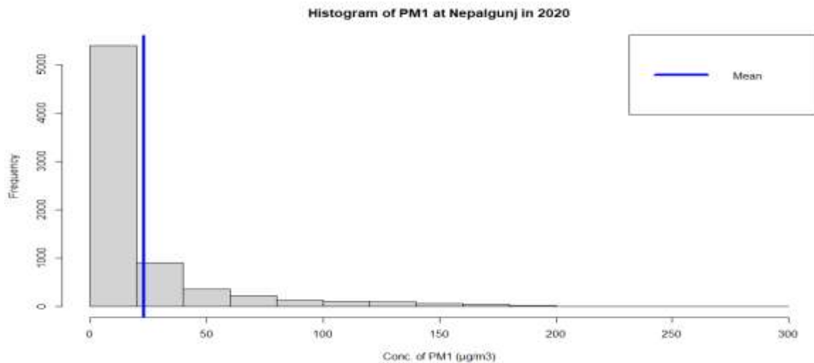
Figure 54 : Histogram for the ambient concentration of PM 1
