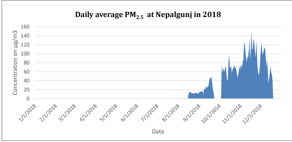
Figure 8: Daily average of PM 2.5 in 2018
