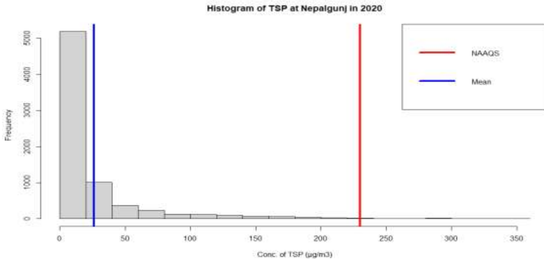
Figure 74: Histogram for the ambient concentration of TSP
