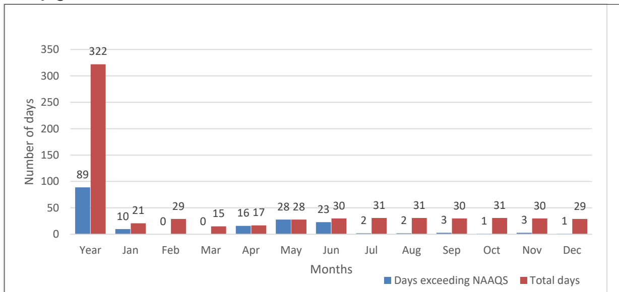
Figure 52: Compliance status of TSP
