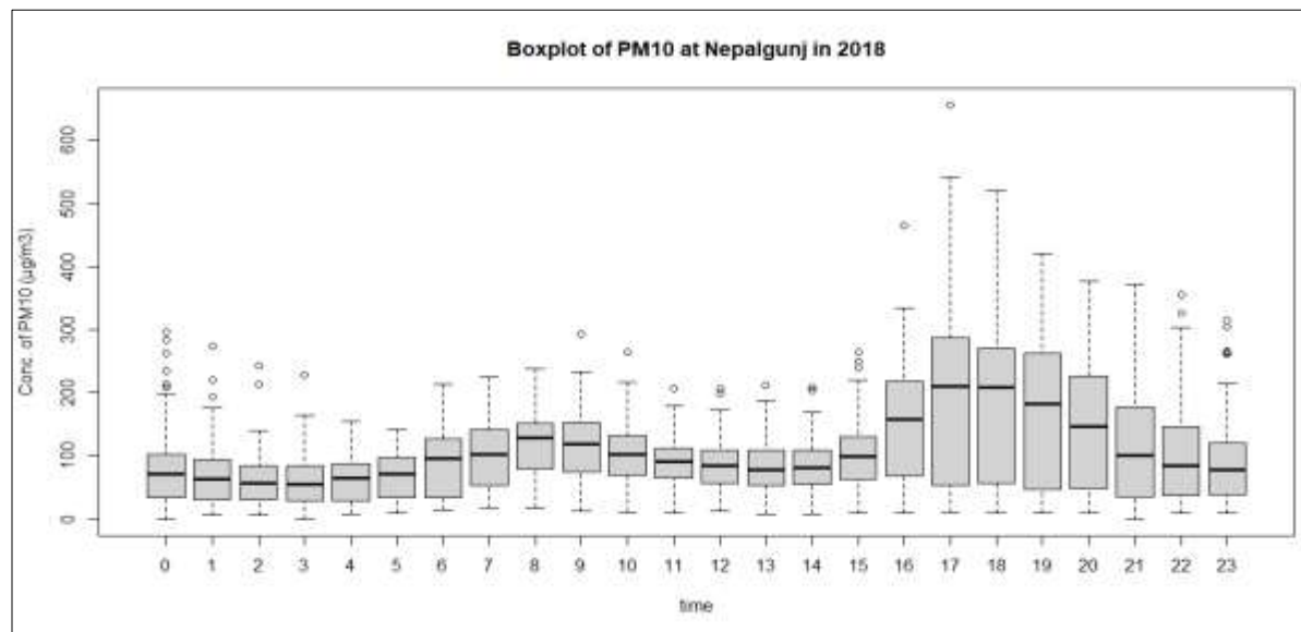
Figure 17: Diurnal variation of average PM 10 concentration
