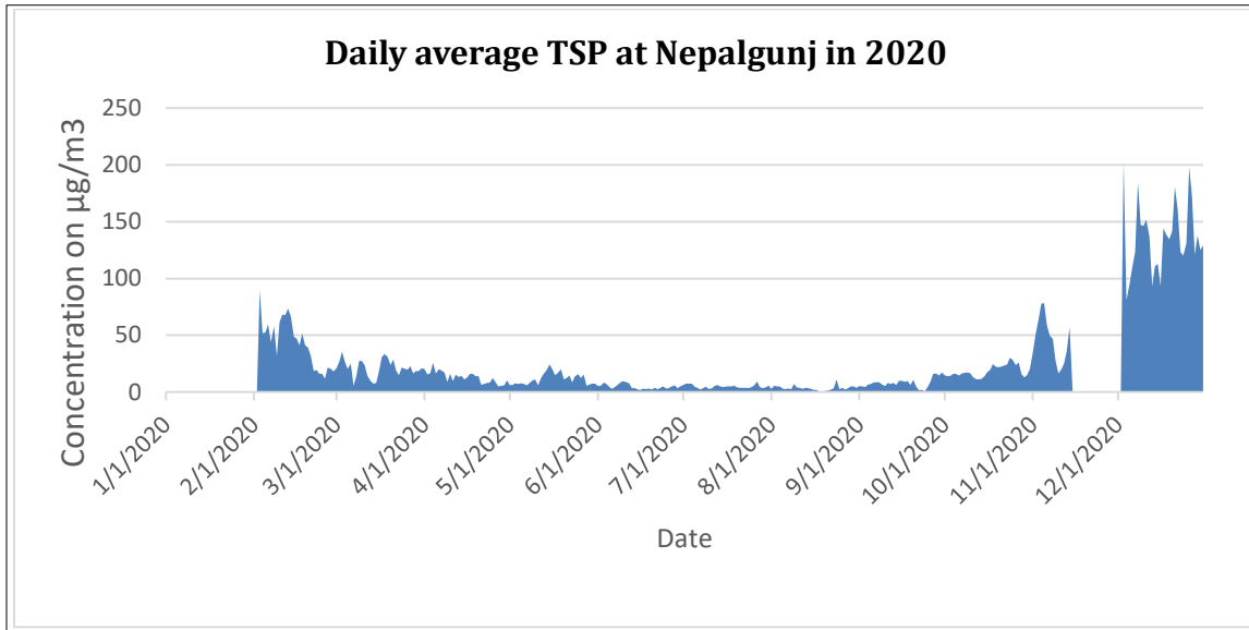
Figure 75: Daily average of TSP
