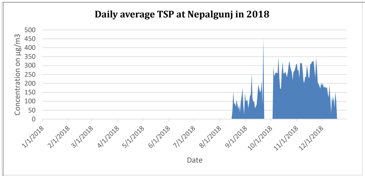
Figure 20: Daily average of TSP in 2018
