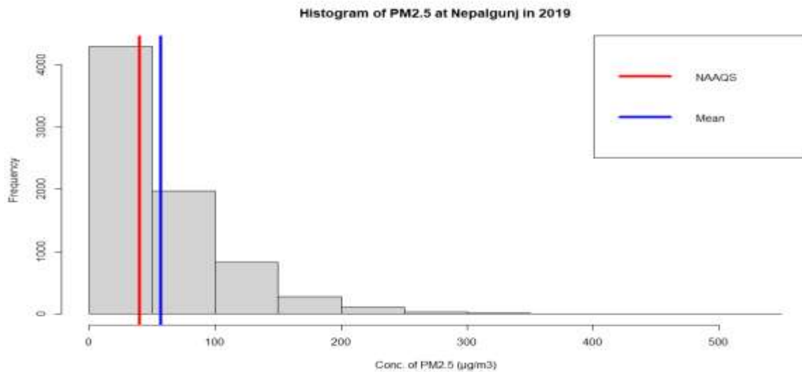
Figure 32 : Histogram for the ambient concentration of PM 2.5
