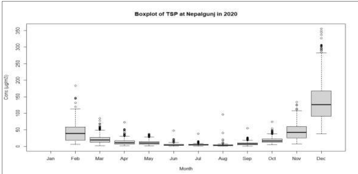
Figure 77: Monthly Variation of TSP
