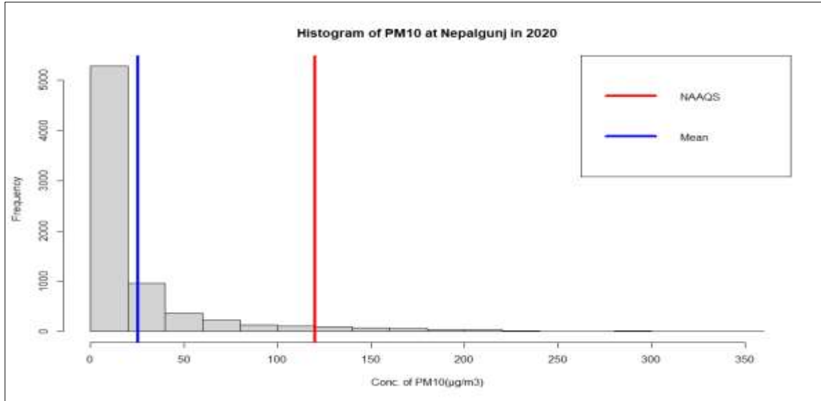
Figure 67: Histogram for the ambient concentration of PM 10
