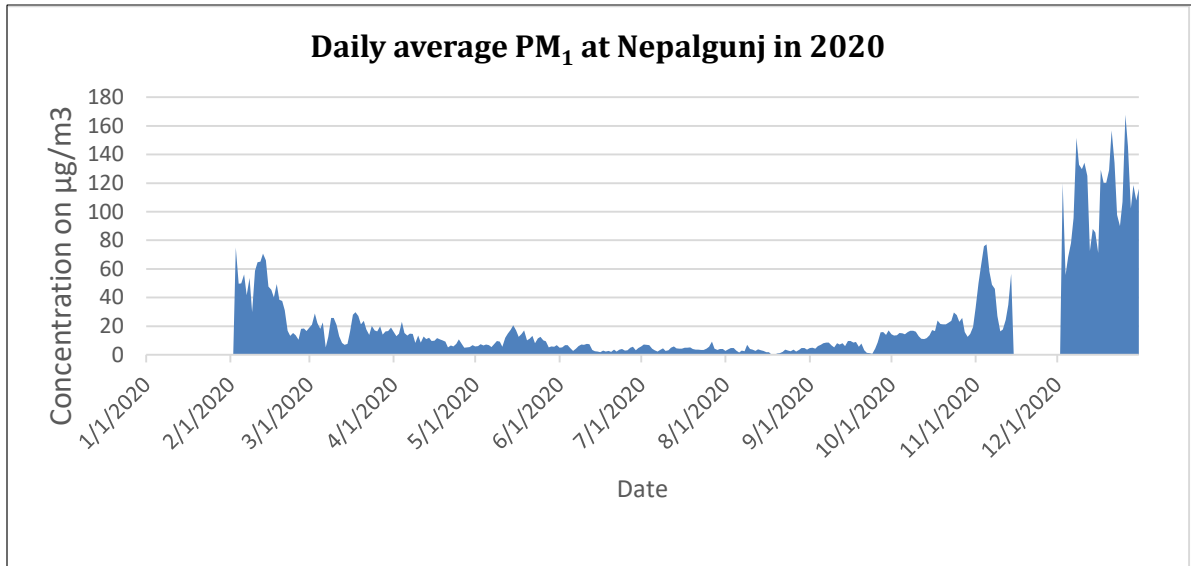
Figure 55: Daily average of PM 1
