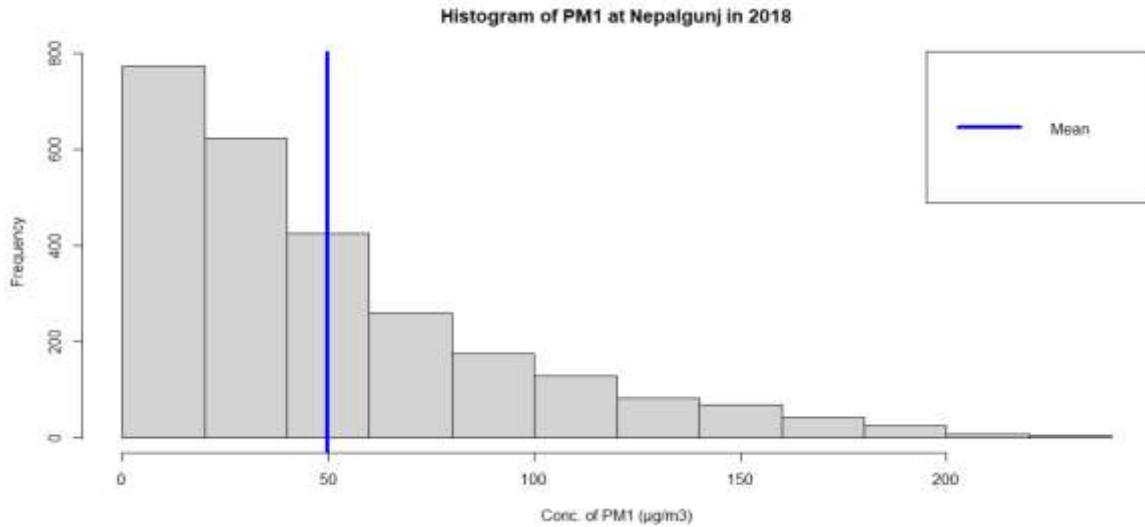
Figure 2 : Histogram for the ambient concentration of PM 1
