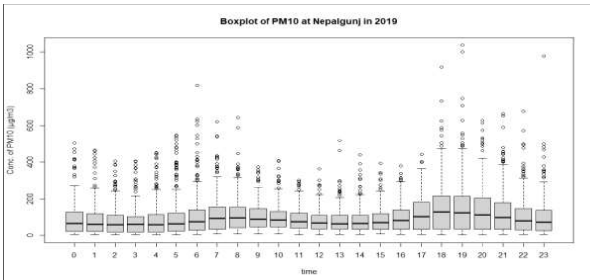
Figure 44: Diurnal variation of average PM 10 concentration
