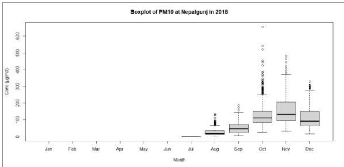
Figure 16: Monthly Variation of PM 10
