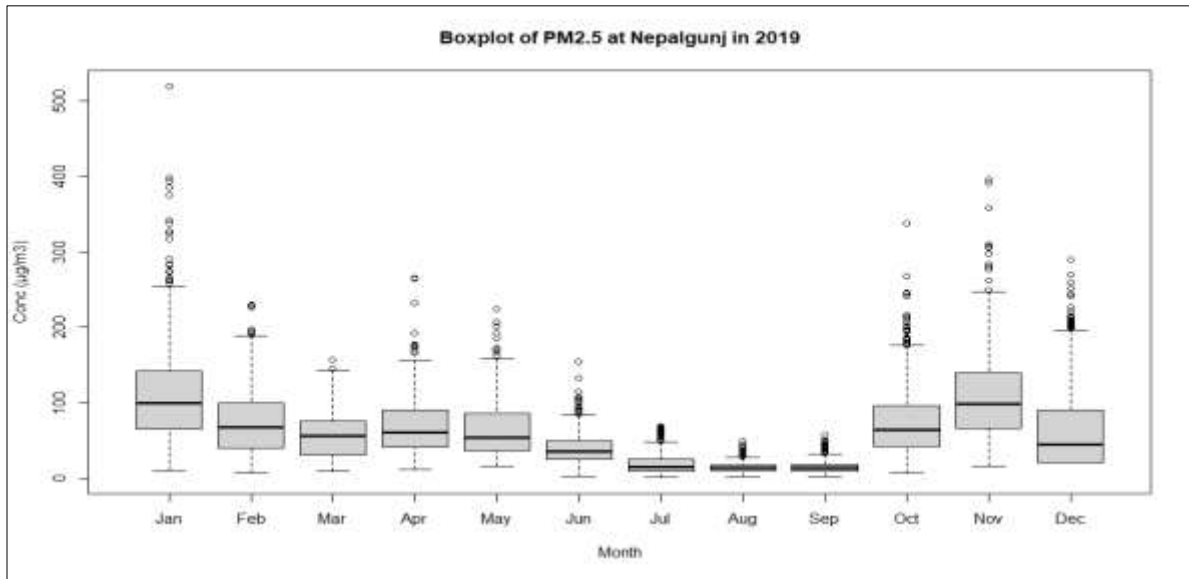
Figure 35: Monthly Variation of PM 2.5
