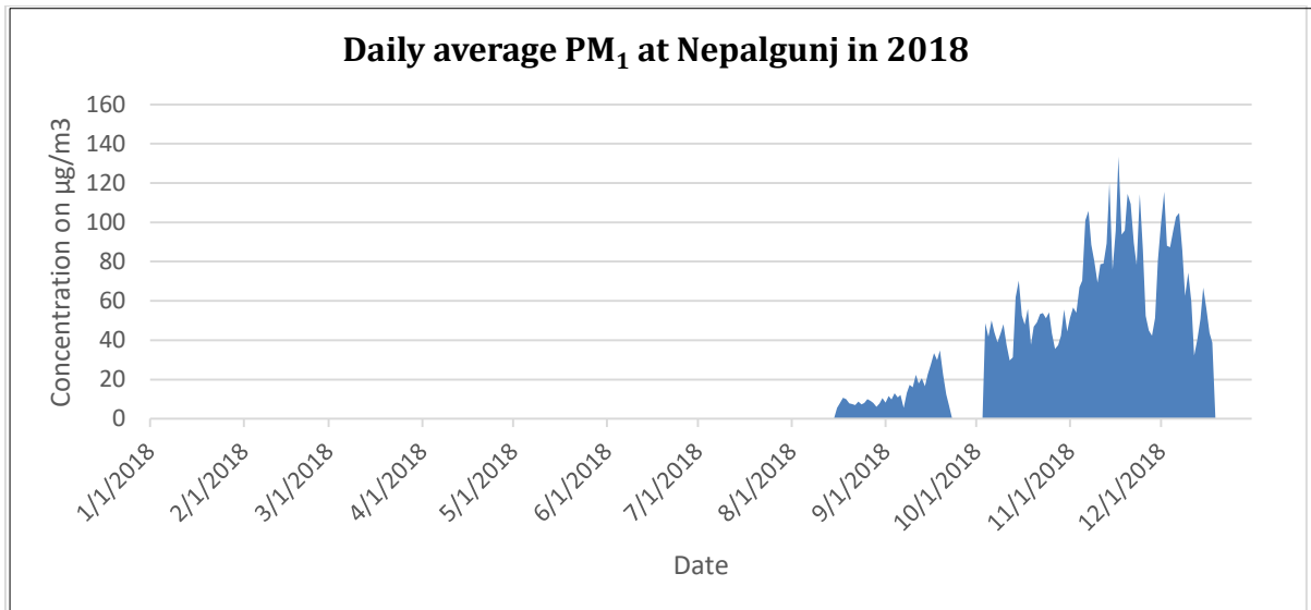
Figure 3: Daily average of PM 1
