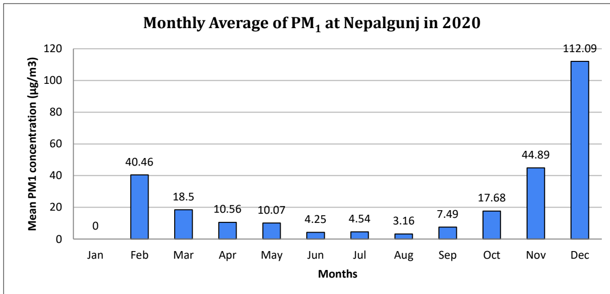
Figure 56: Monthly average of PM 1
