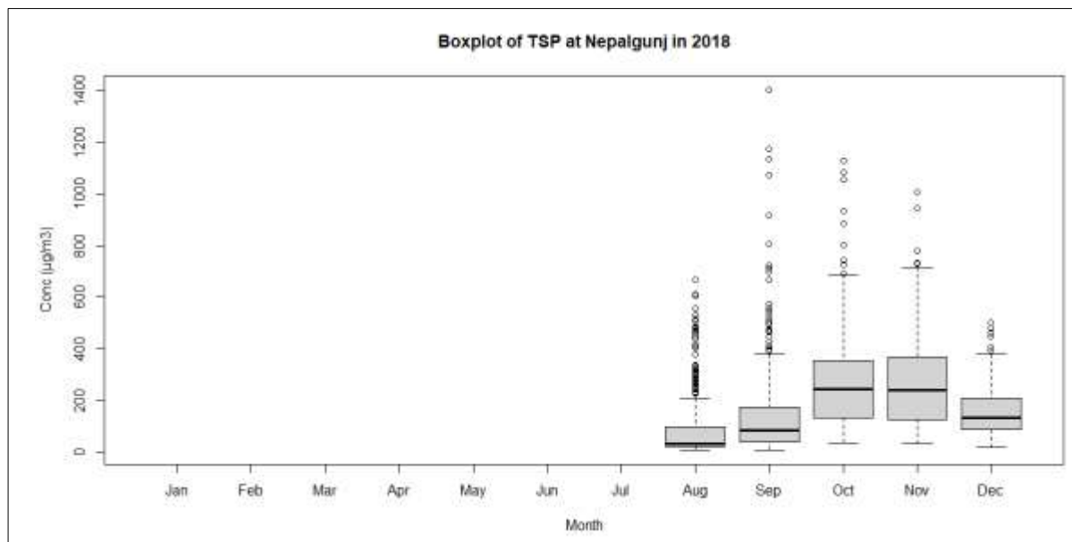
Figure 22: Monthly Variation of TSP
