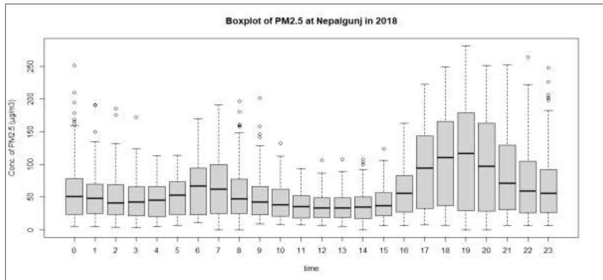
Figure 11: Diurnal variation of average PM 2.5 concentration
