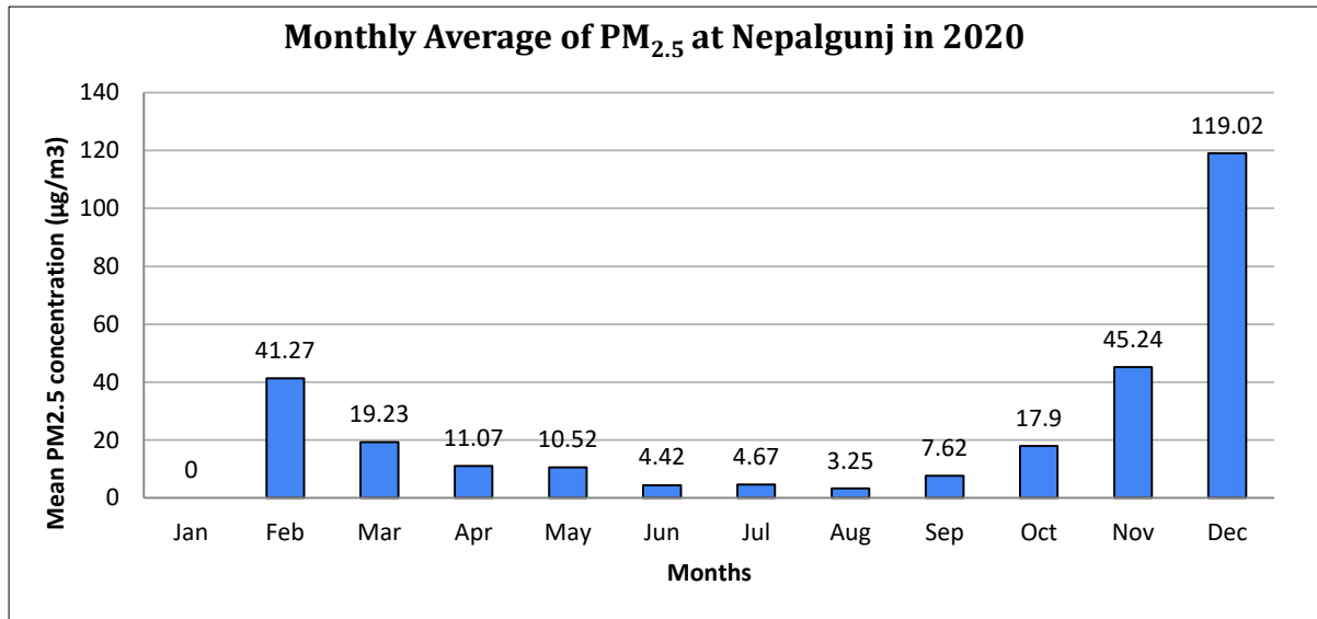
Figure 62: Monthly average of PM 2.5
