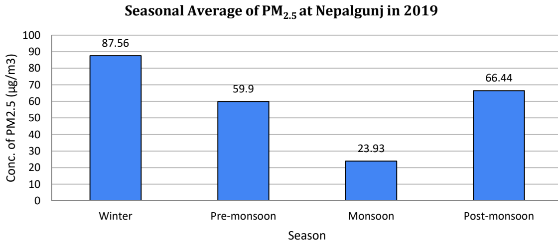
Figure 36: Seasonal variation of PM 2.5
