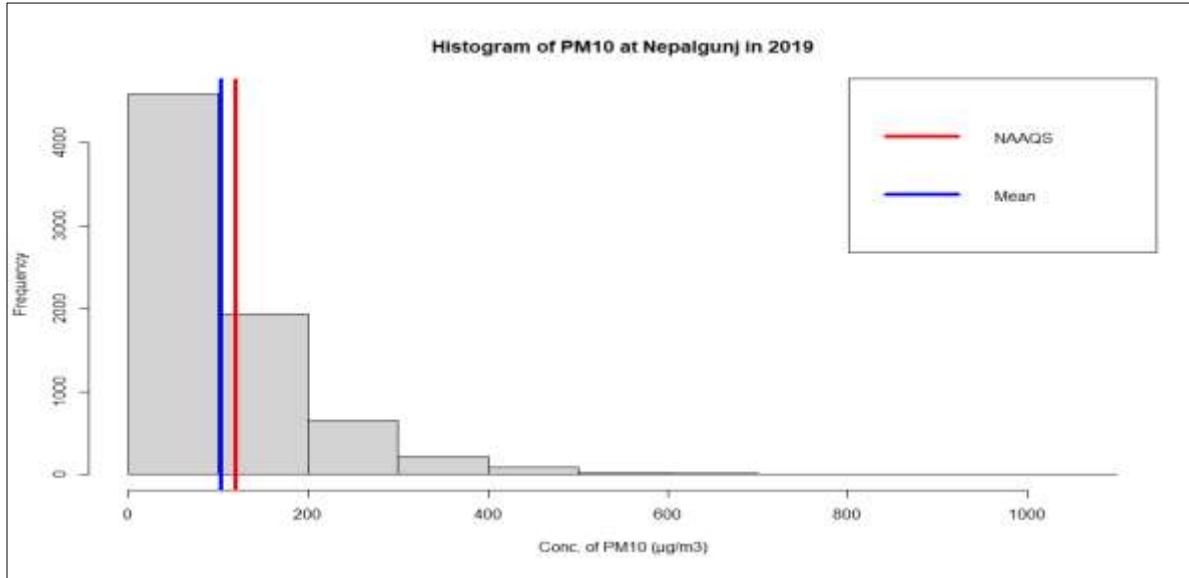
Figure 39: Histogram for the ambient concentration of PM 10
