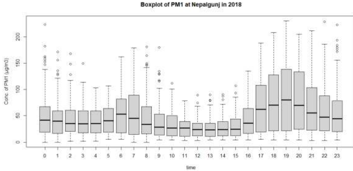
Figure 6: Diurnal variation of average PM 1 concentration
