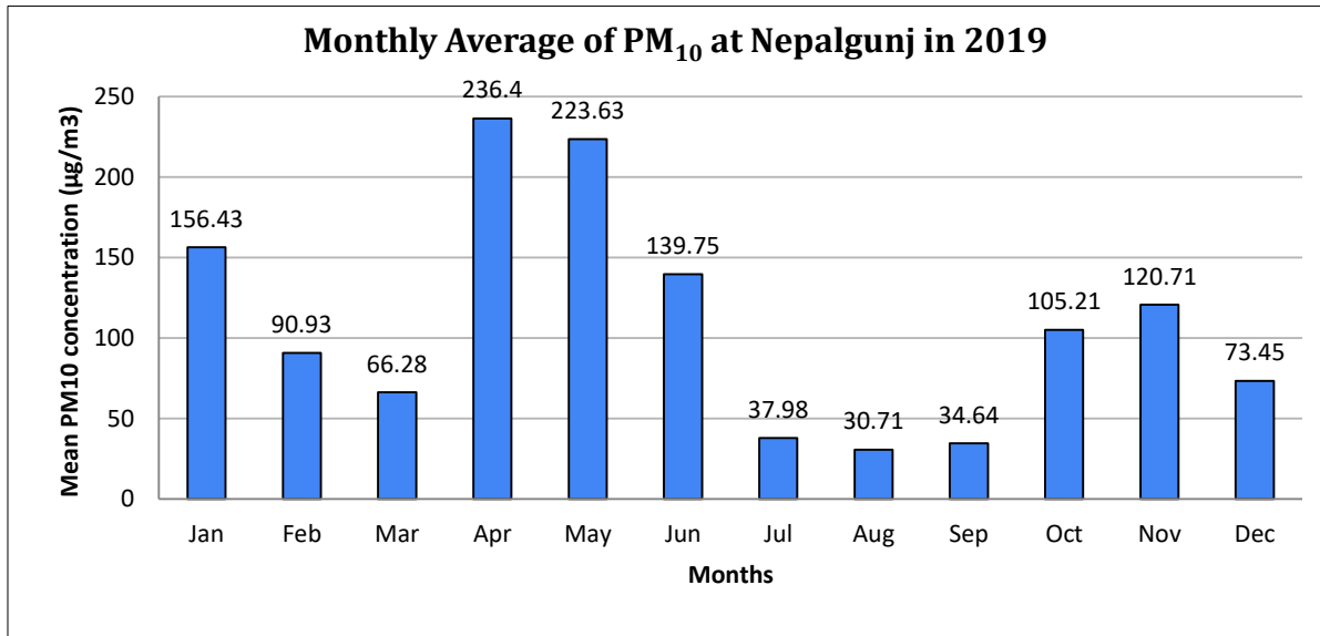
Figure 41: Monthly average of PM 10
