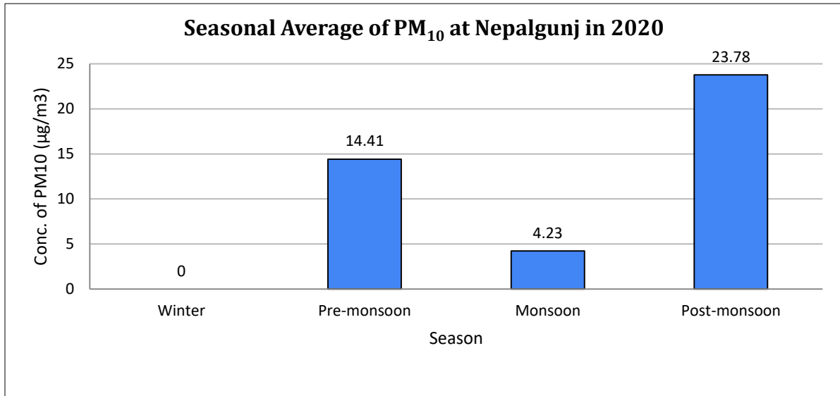
Figure 71: Seasonal variation of PM 10
