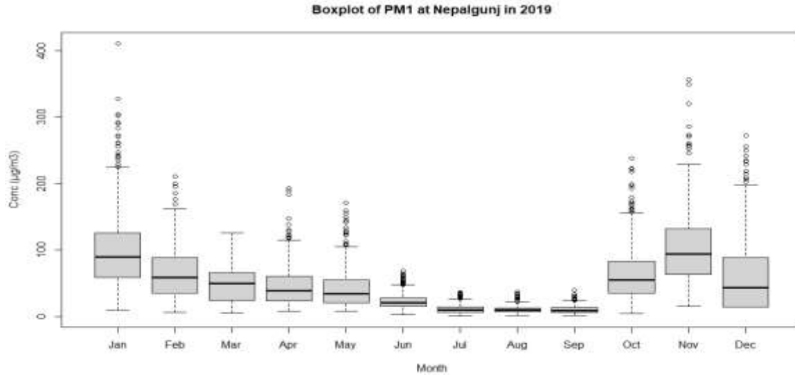
Figure 29: Monthly Variation of PM 1
