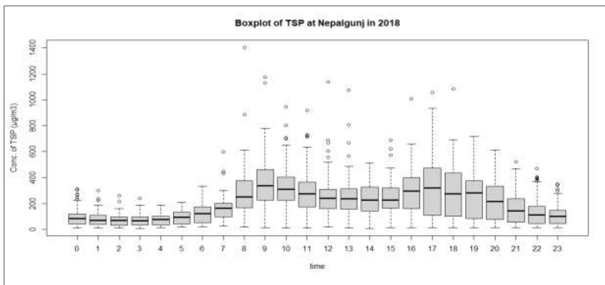
Figure 23: Diurnal variation of average TSP concentration
