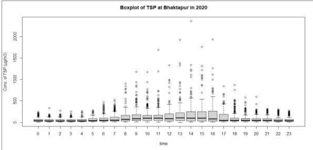
Figure 79: Diurnal variation of average TSP concentration
