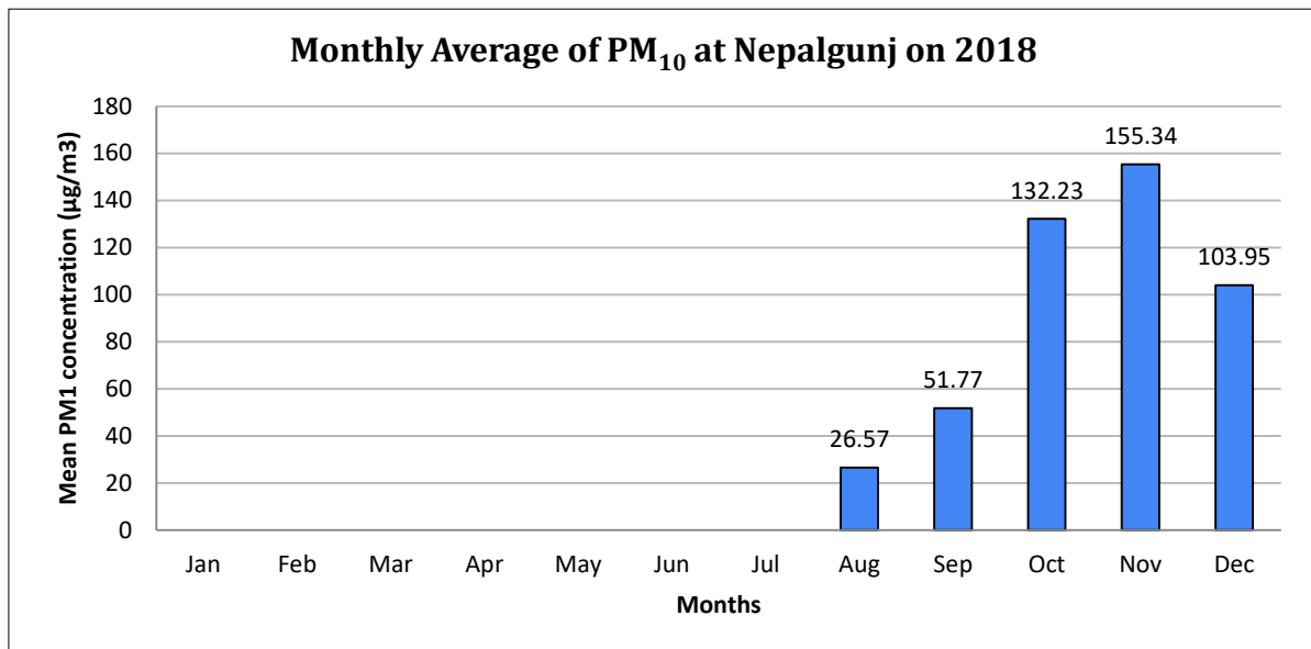
Figure 15: Monthly average of PM 10
