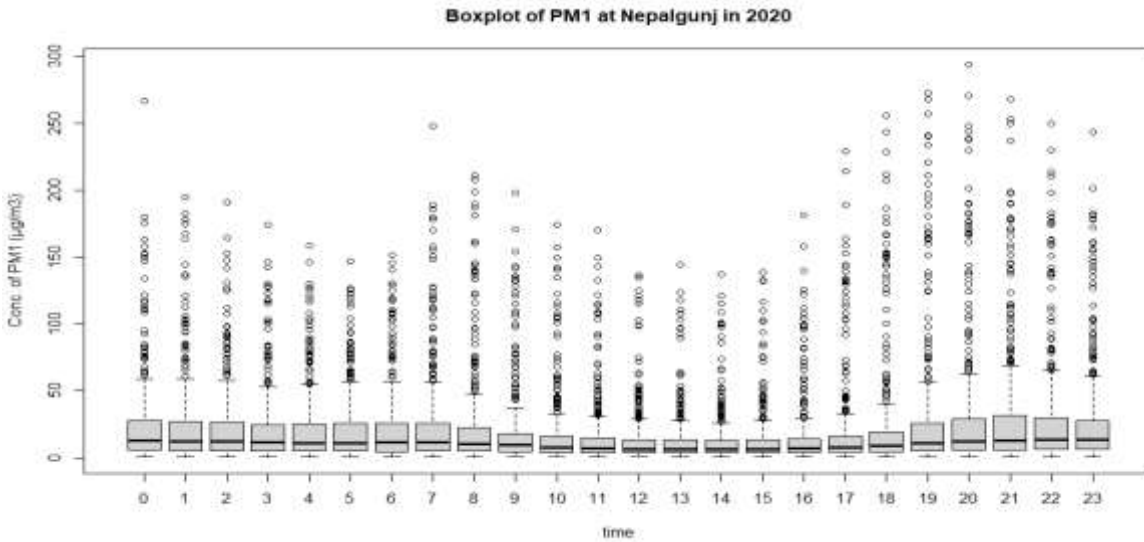
Figure 59: Diurnal variation of average PM 1 concentration
